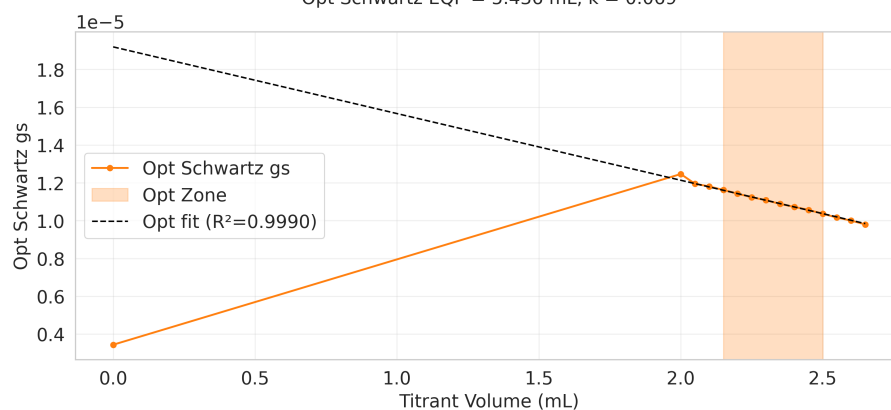
Opt Schwartz EQP = 5.436 mL, k = 0.069
