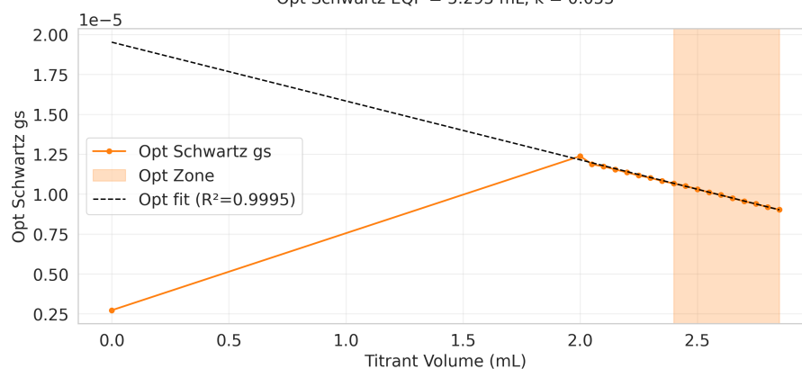
Opt Schwartz EQP = 5.295 mL, k = 0.055
