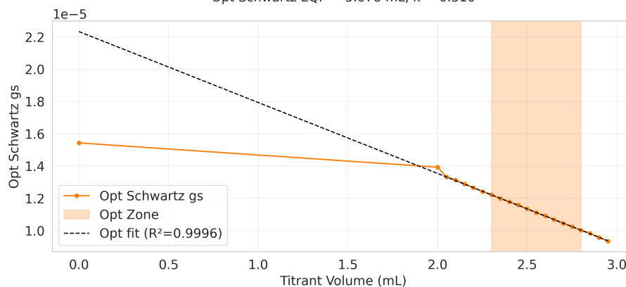
Opt Schwartz EQP = 5.078 mL, k = 0.310
