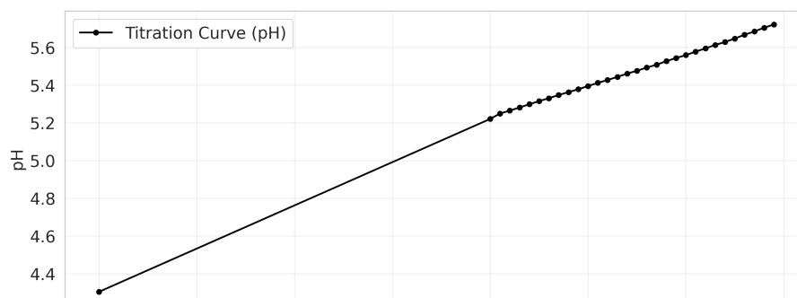
Opt Schwartz EQP = 5.090 mL, k = 0.268
