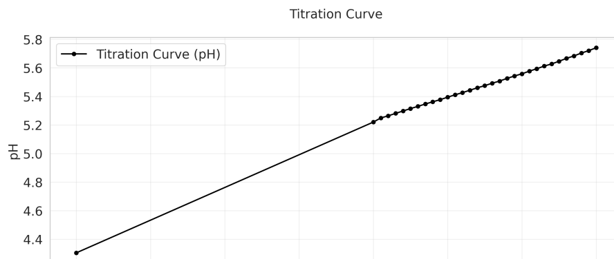
Opt Schwartz EQP = 5.055 mL, k = 0.348
