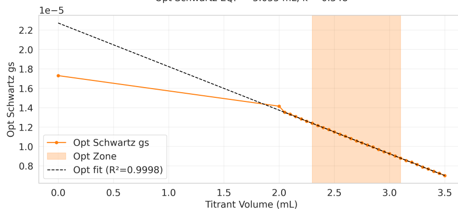
Opt Schwartz EQP = 5.055 mL, k = 0.348
