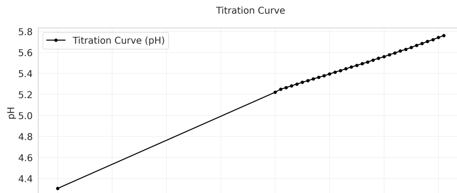
Opt Schwartz EQP = 5.100 mL, k = 0.276
