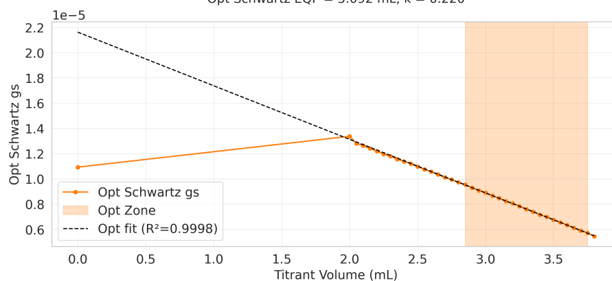
Opt Schwartz EQP = 5.092 mL, k = 0.220
