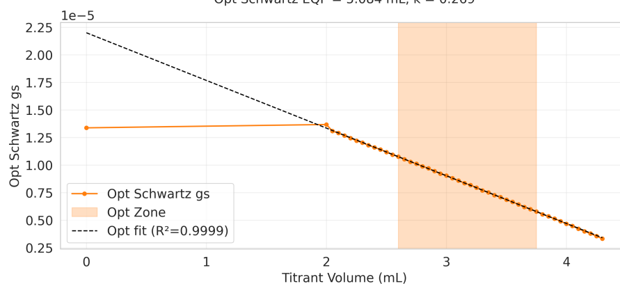
Opt Schwartz EQP = 5.084 mL, k = 0.269
