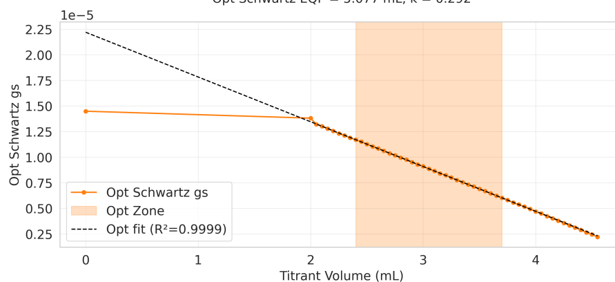
Opt Schwartz EQP = 5.077 mL, k = 0.292
