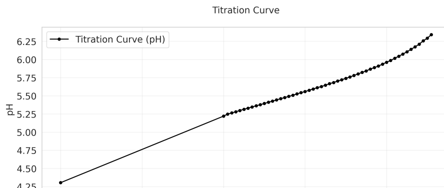
Opt Schwartz EQP = 5.077 mL, k = 0.292
