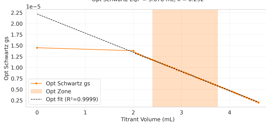
Opt Schwartz EQP = 5.078 mL, k = 0.292
