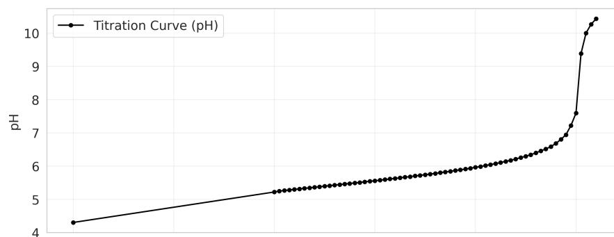
Opt Schwartz EQP = 5.031 mL, k = 0.567
