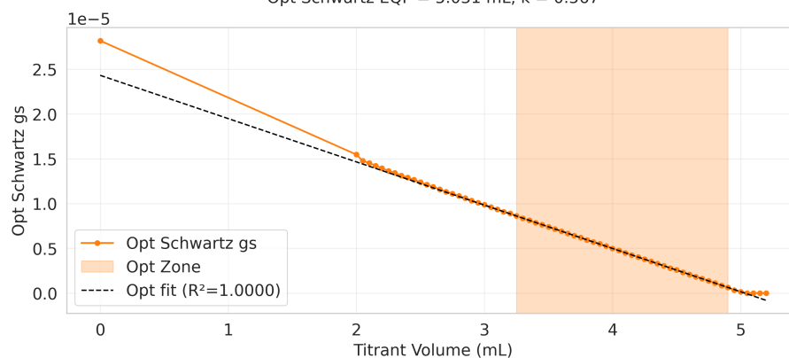
Opt Schwartz EQP = 5.031 mL, k = 0.567
