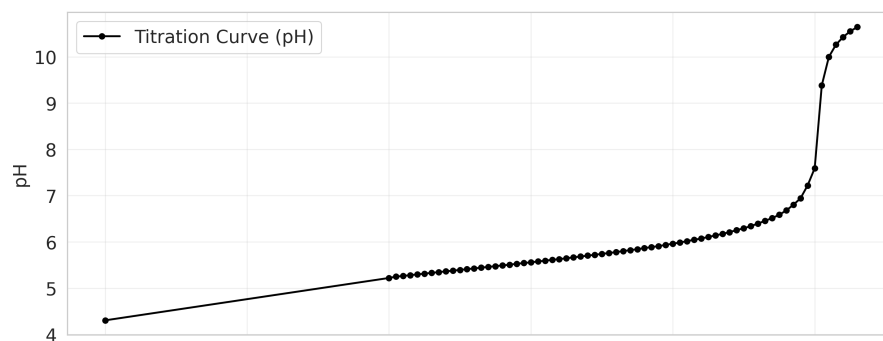
Opt Schwartz EQP = 5.029 mL, k = 0.610
