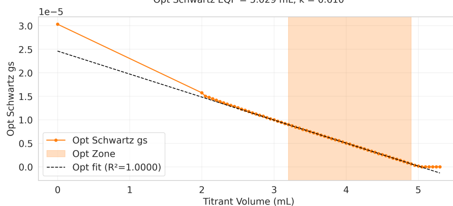
Opt Schwartz EQP = 5.029 mL, k = 0.610
