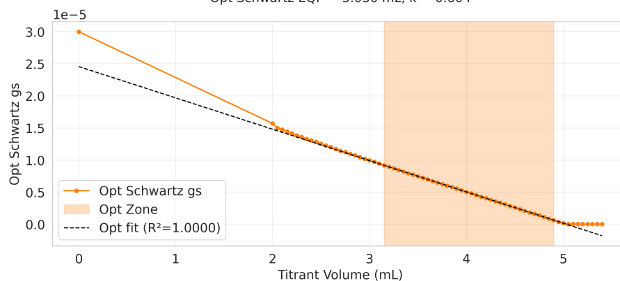
Opt Schwartz EQP = 5.030 mL, k = 0.604
