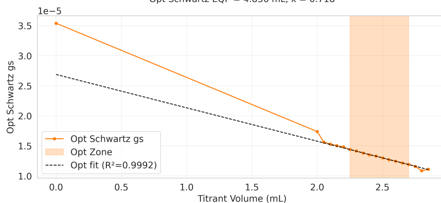
Opt Schwartz EQP = 4.836 mL, k = 0.718
