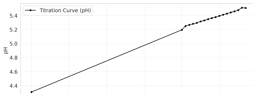
Opt Schwartz EQP = 4.836 mL, k = 0.718
