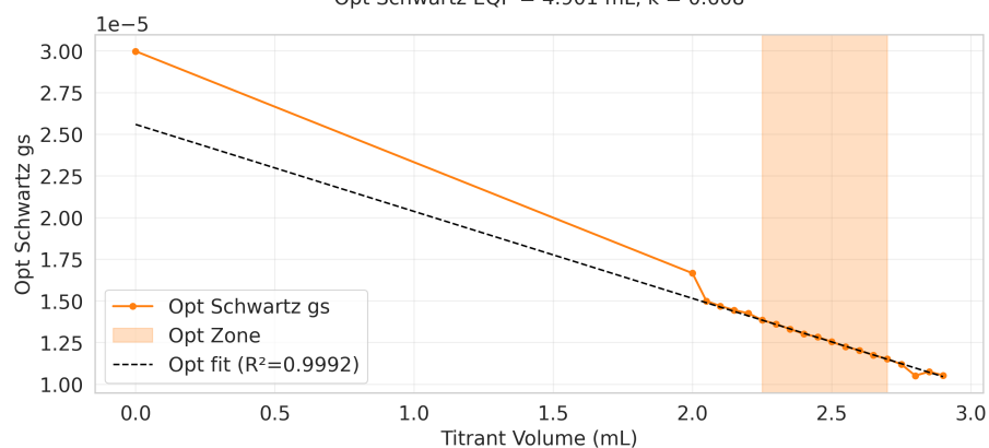
Opt Schwartz EQP = 4.901 mL, k = 0.608
