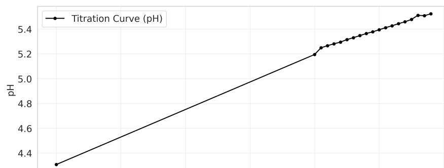
Opt Schwartz EQP = 4.901 mL, k = 0.608
