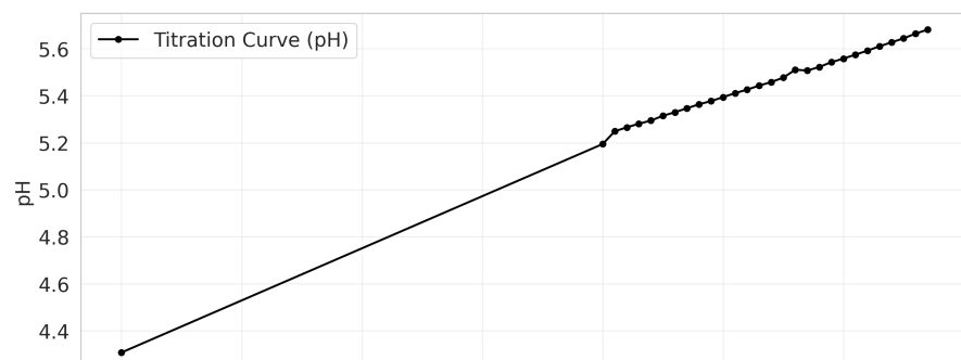
Opt Schwartz EQP = 4.979 mL, k = 0.405
