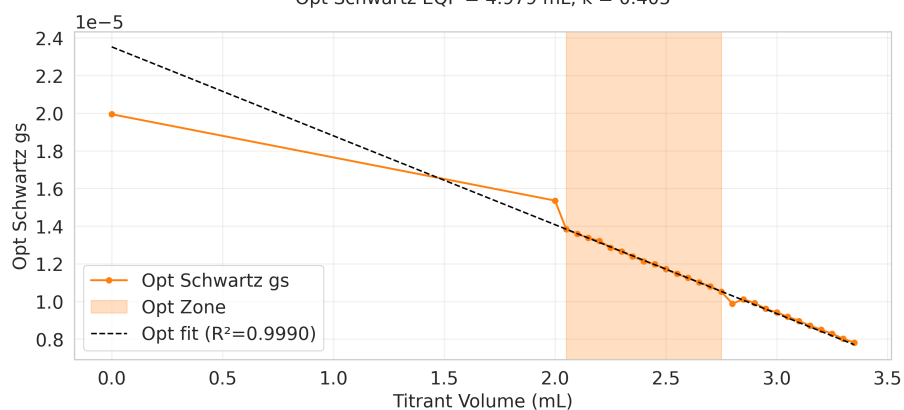
Opt Schwartz EQP = 4.979 mL, k = 0.405
