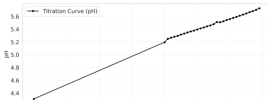
Opt Schwartz EQP = 4.933 mL, k = 0.460
