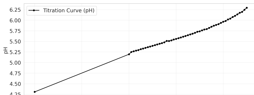
Opt Schwartz EQP = 5.050 mL, k = 0.422
