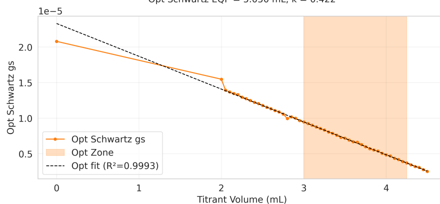
Opt Schwartz EQP = 5.050 mL, k = 0.422
