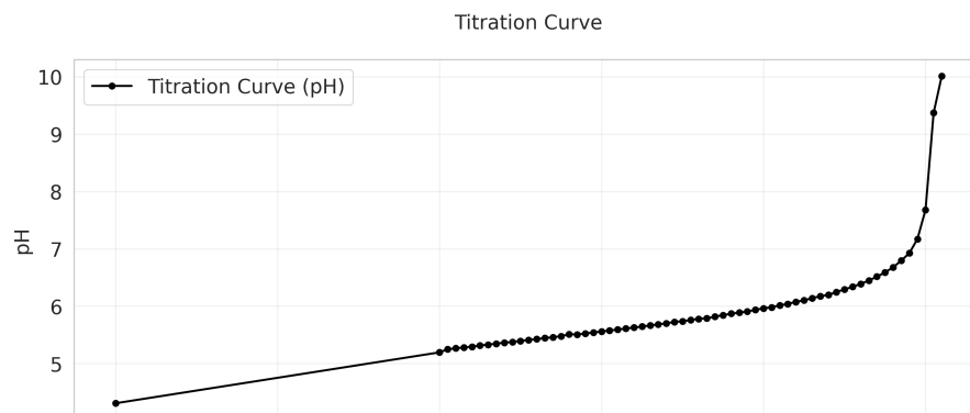
Opt Schwartz EQP = 5.033 mL, k = 0.561
