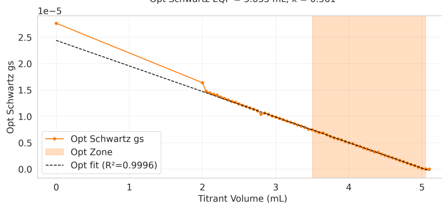
Opt Schwartz EQP = 5.033 mL, k = 0.561
