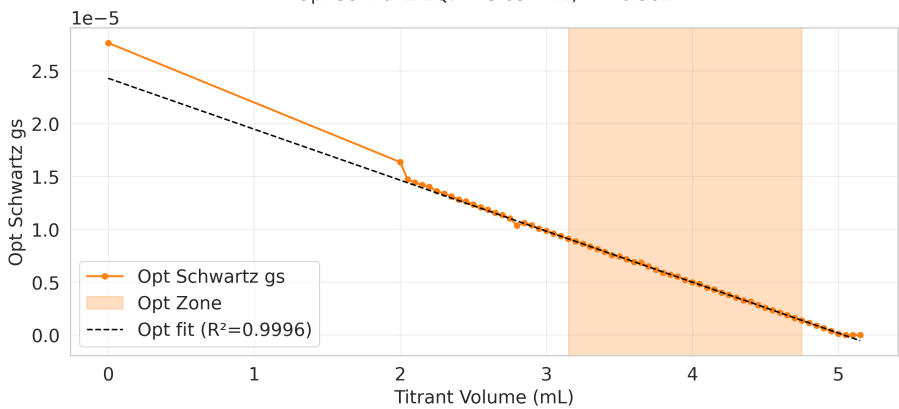
Opt Schwartz EQP = 5.037 mL, k = 0.561
