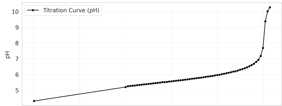
Opt Schwartz EQP = 5.037 mL, k = 0.561
