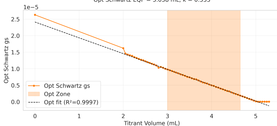
Opt Schwartz EQP = 5.038 mL, k = 0.533
