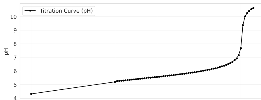
Opt Schwartz EQP = 5.038 mL, k = 0.533
