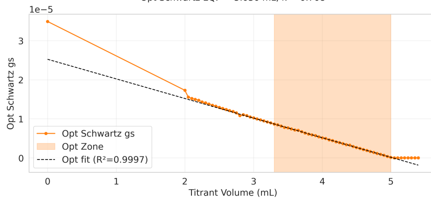
Opt Schwartz EQP = 5.030 mL, k = 0.708
