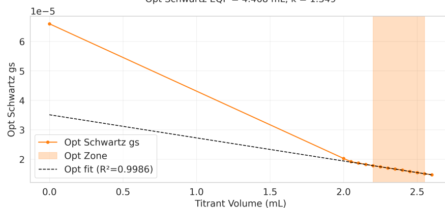
Opt Schwartz EQP = 4.468 mL, k = 1.349
