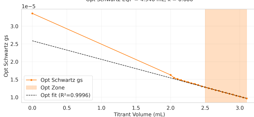
Opt Schwartz EQP = 4.946 mL, k = 0.686
