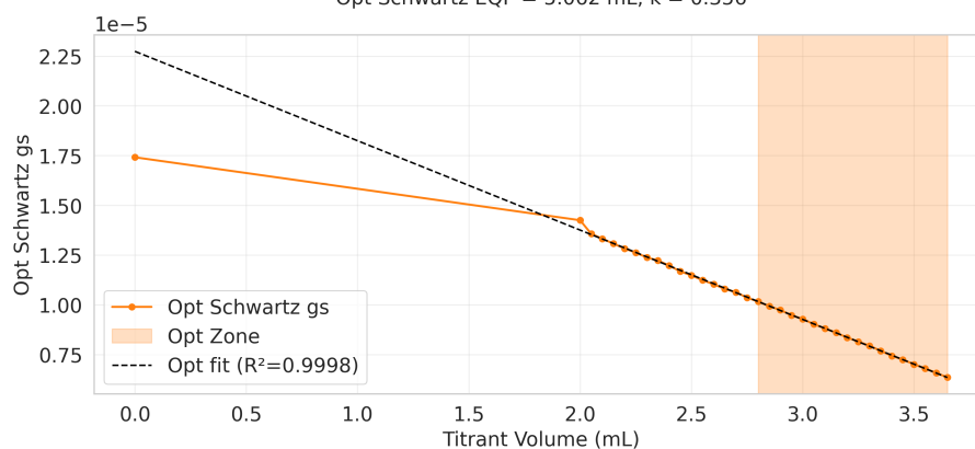
Opt Schwartz EQP = 5.062 mL, k = 0.356
