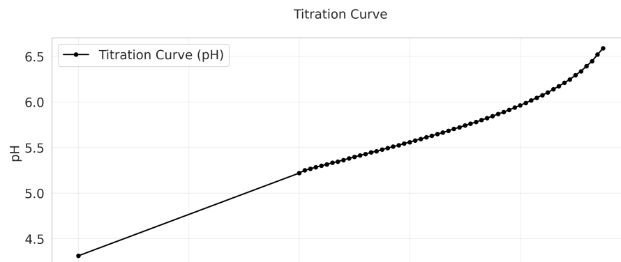
Opt Schwartz EQP = 5.045 mL, k = 0.443
