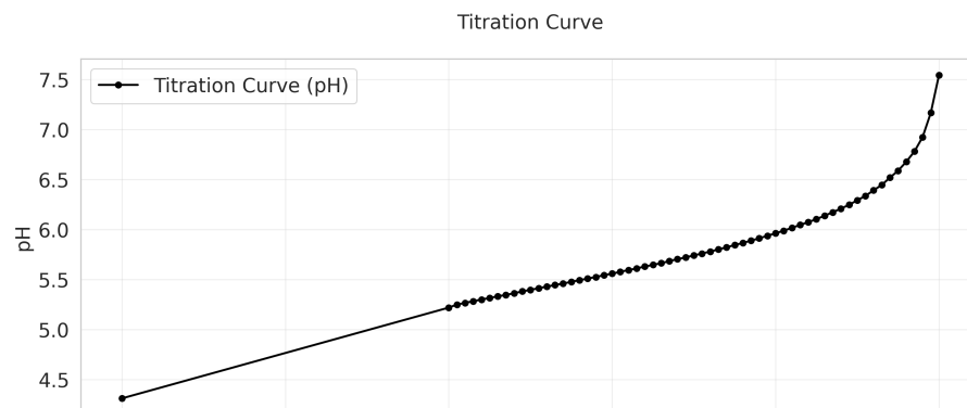
Opt Schwartz EQP = 5.043 mL, k = 0.450
