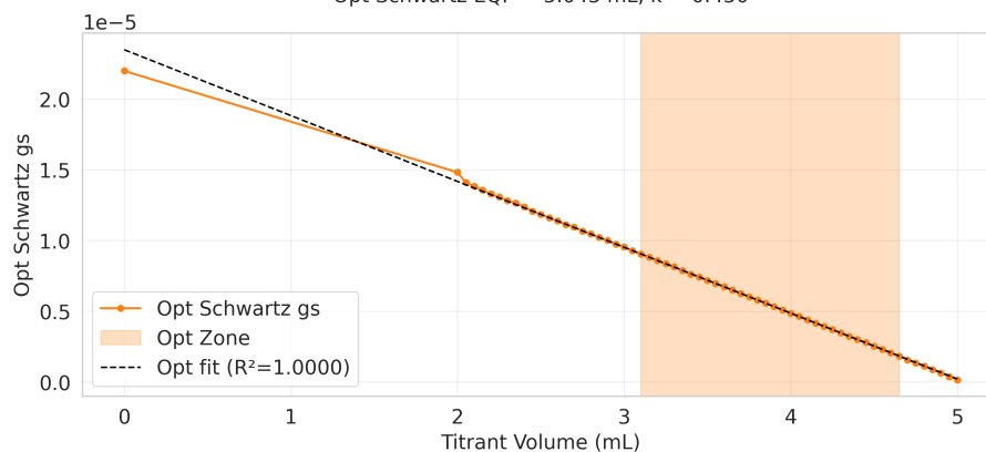
Opt Schwartz EQP = 5.043 mL, k = 0.450
