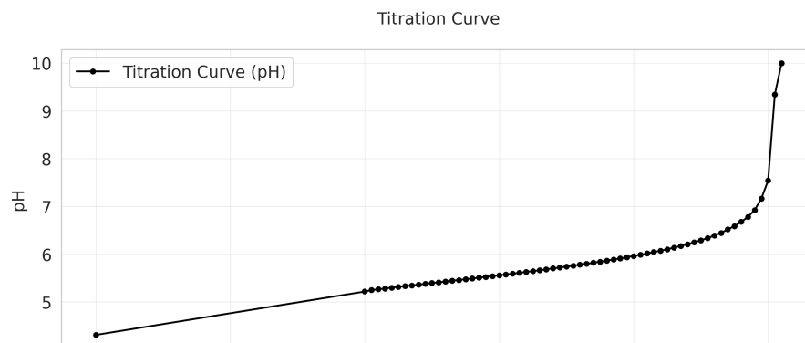
Opt Schwartz EQP = 5.036 mL, k = 0.557
