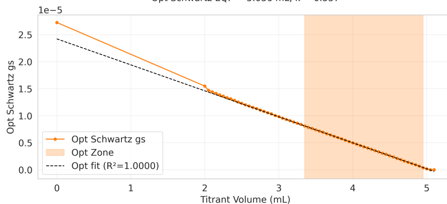
Opt Schwartz EQP = 5.036 mL, k = 0.557
