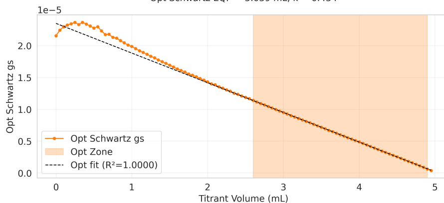
Opt Schwartz EQP = 5.039 mL, k = 0.434
