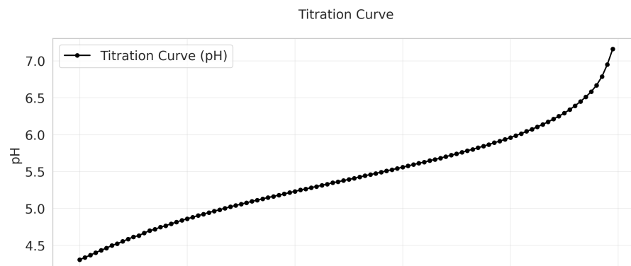
Opt Schwartz EQP = 5.039 mL, k = 0.434
