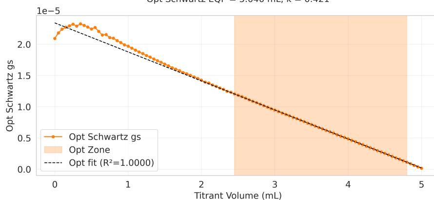
Opt Schwartz EQP = 5.040 mL, k = 0.421
