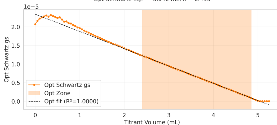
Opt Schwartz EQP = 5.040 mL, k = 0.416
