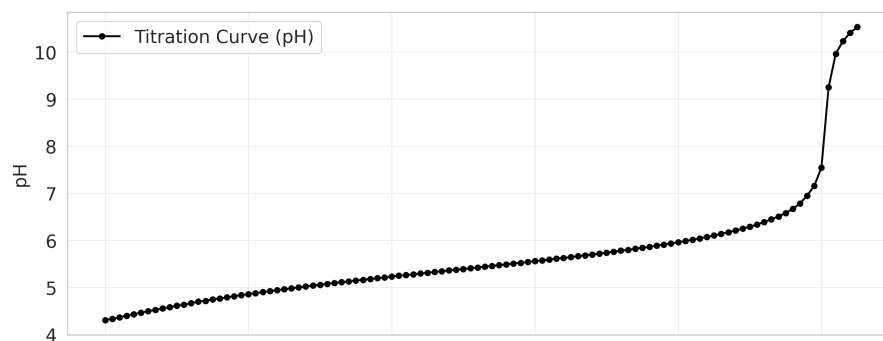
Opt Schwartz EQP = 5.040 mL, k = 0.416
