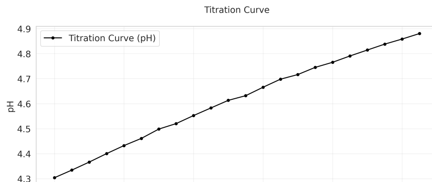
Opt Schwartz EQP = nan mL, k = 0.749
