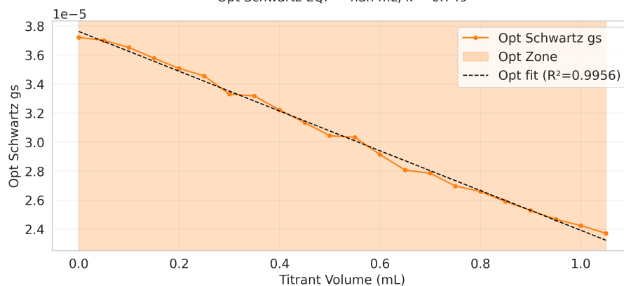
Opt Schwartz EQP = nan mL, k = 0.749
