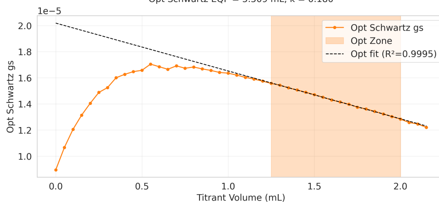
Opt Schwartz EQP = 5.509 mL, k = 0.180
