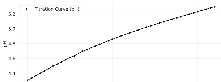
Opt Schwartz EQP = 5.335 mL, k = 0.221
