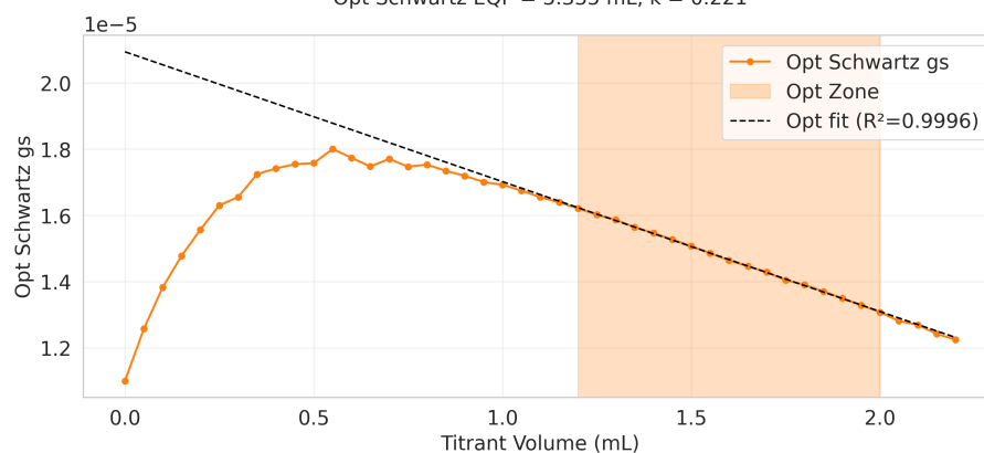
Opt Schwartz EQP = 5.335 mL, k = 0.221
