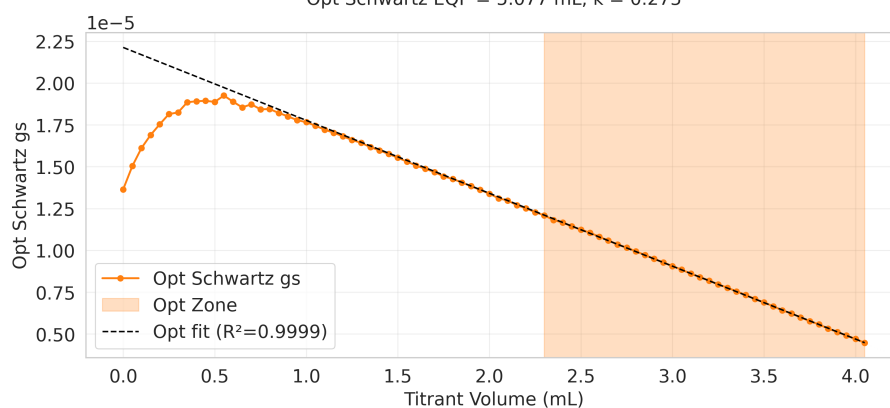
Opt Schwartz EQP = 5.077 mL, k = 0.275
