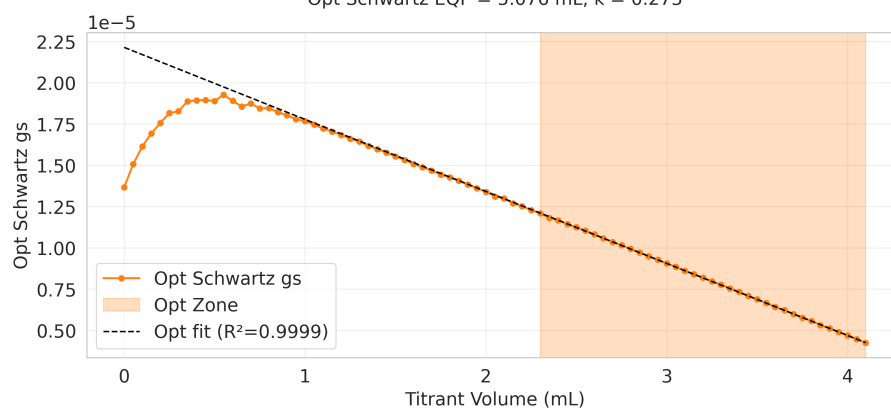
Opt Schwartz EQP = 5.076 mL, k = 0.275
