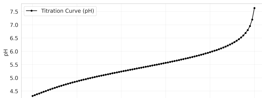
Opt Schwartz EQP = 5.035 mL, k = 0.453
