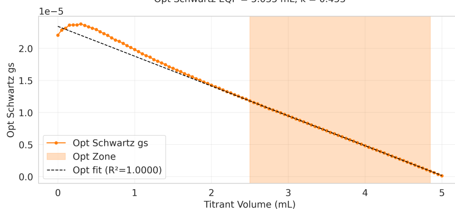
Opt Schwartz EQP = 5.035 mL, k = 0.453
