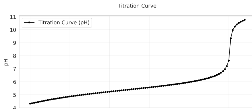
Opt Schwartz EQP = 5.032 mL, k = 0.459
