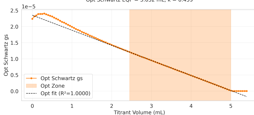
Opt Schwartz EQP = 5.032 mL, k = 0.459
