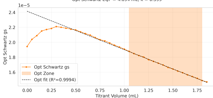
Opt Schwartz EQP = 4.694 mL, k = 0.399
