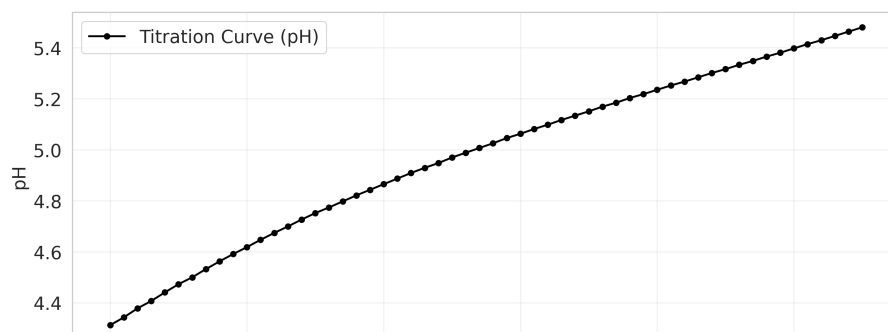
Opt Schwartz EQP = 4.976 mL, k = 0.367
