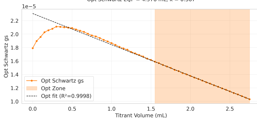
Opt Schwartz EQP = 4.976 mL, k = 0.367
