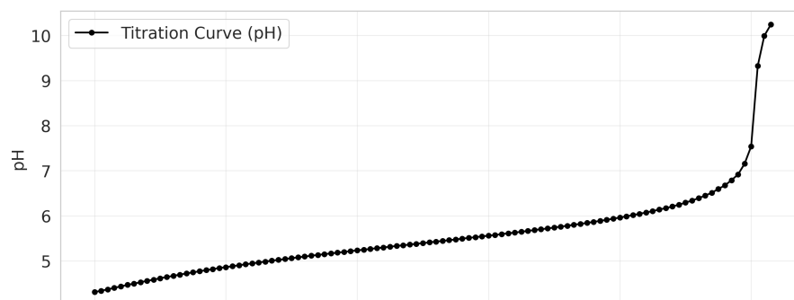
Opt Schwartz EQP = 5.036 mL, k = 0.503
