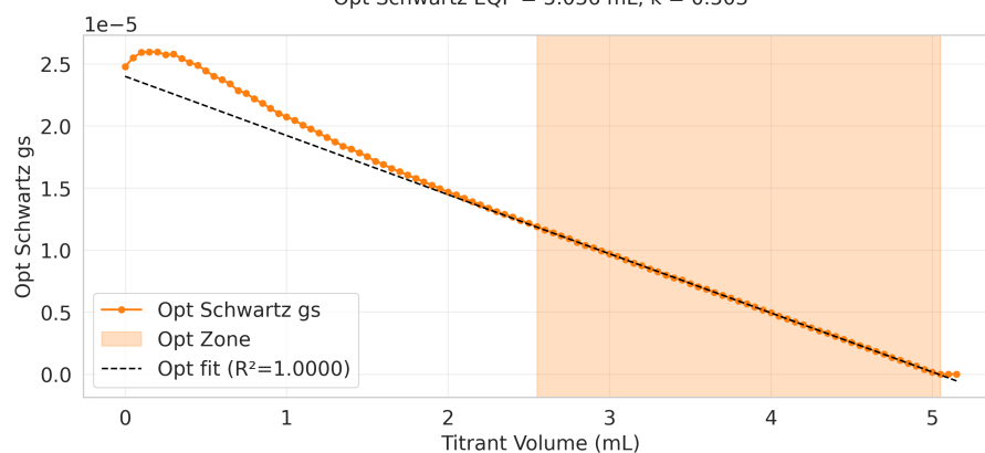
Opt Schwartz EQP = 5.036 mL, k = 0.503
