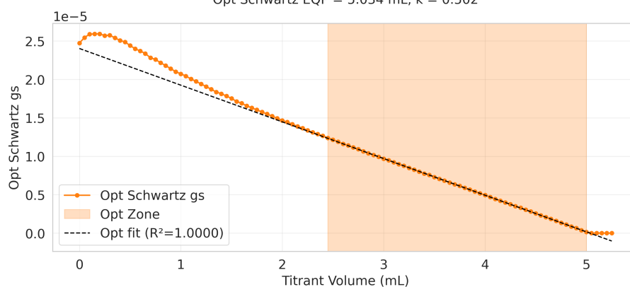
Opt Schwartz EQP = 5.034 mL, k = 0.502
