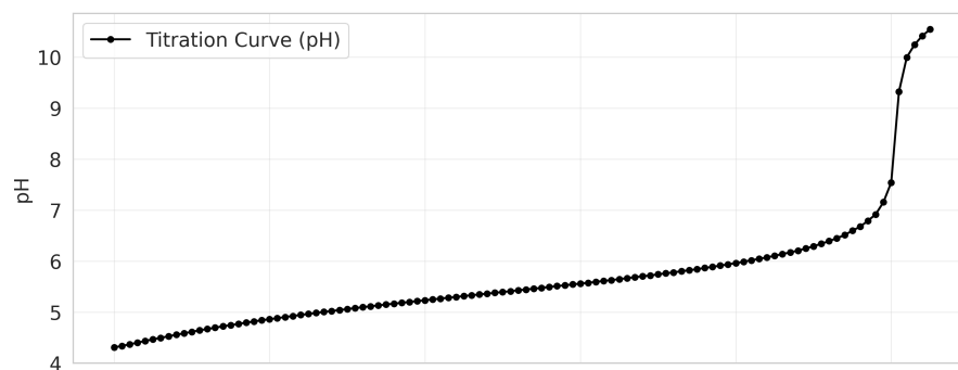
Opt Schwartz EQP = 5.034 mL, k = 0.502
