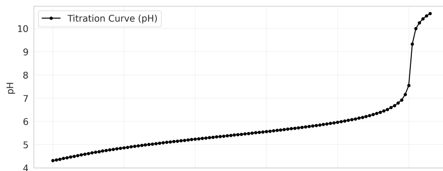
Opt Schwartz EQP = 5.034 mL, k = 0.498
