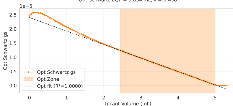
Opt Schwartz EQP = 5.034 mL, k = 0.498
