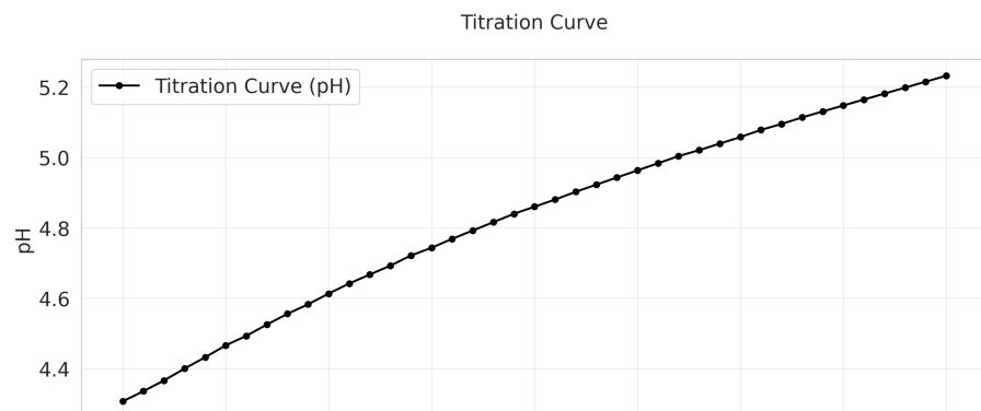
Opt Schwartz EQP = 5.698 mL, k = 0.108
