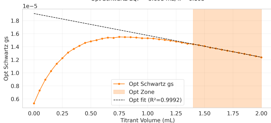
Opt Schwartz EQP = 5.698 mL, k = 0.108
