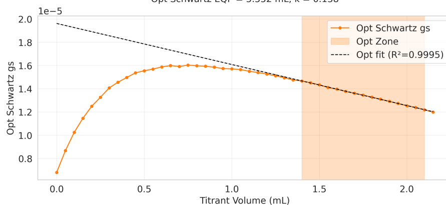
Opt Schwartz EQP = 5.552 mL, k = 0.138
