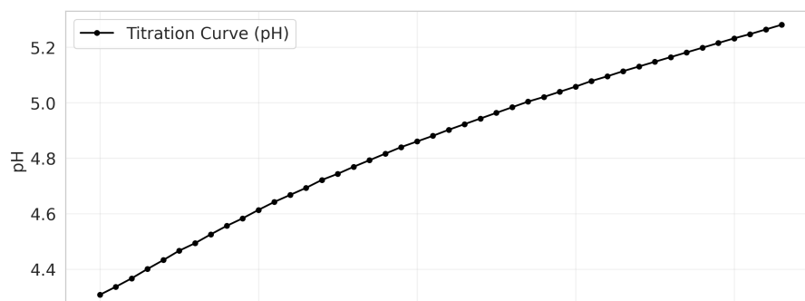
Opt Schwartz EQP = 5.552 mL, k = 0.138
