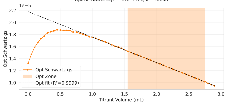
Opt Schwartz EQP = 5.144 mL, k = 0.268
