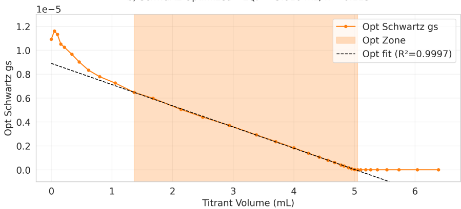
b) Schwartz Optimized - EQP = 5.016 mL, k = 0.113
