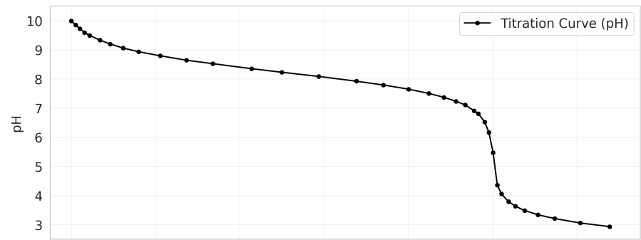
b) Schwartz Optimized - EQP = 5.016 mL, k = 0.113
