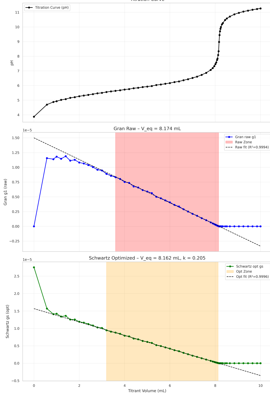
GranTED Analysis Overview Titration Curve
