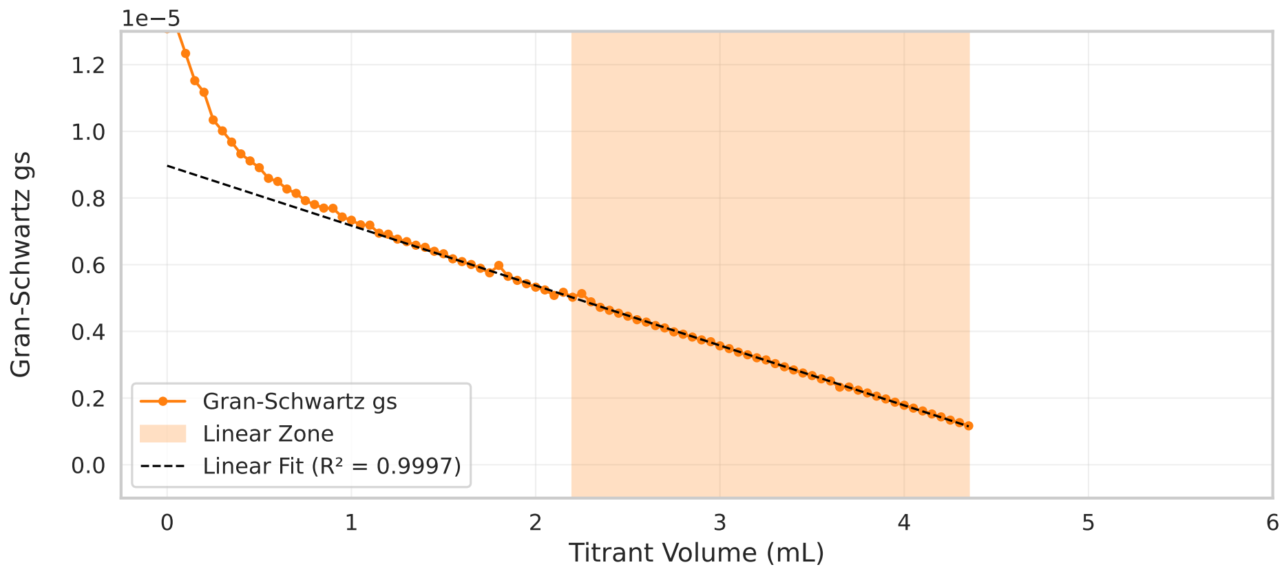
d) Optimised Gran-Schwartz (EQP = 5.002 mL, k = 0.214 )
