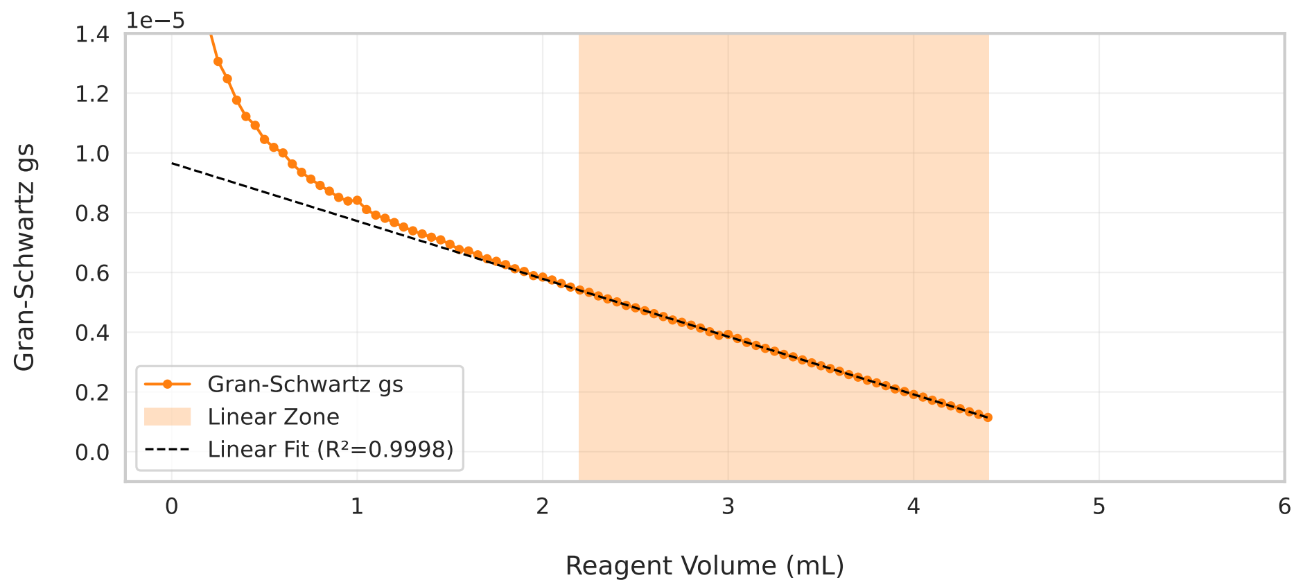
d) Optimised Gran-Schwartz (EQP = 4.990 mL, k = 0.214 )
